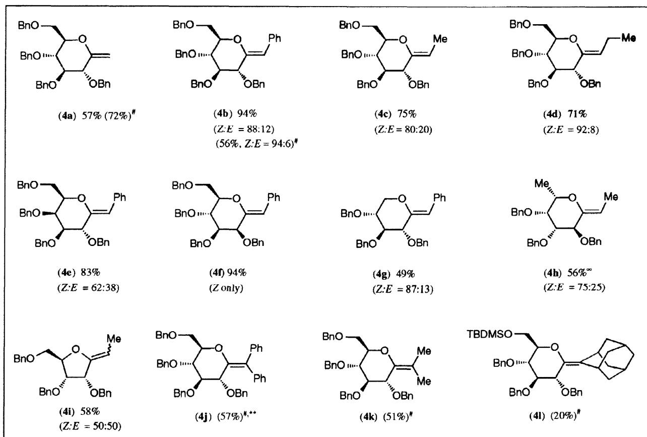
Figure Exo-glycals prepared via the Ramberg-Bäcklund approach* (reactions carried out using \text{CF}_2\text{Br}_2 14 unless otherwise indicated # )
